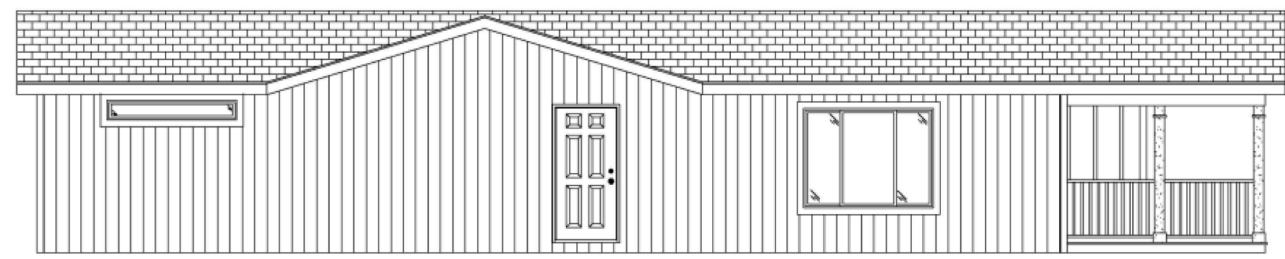
Left Elevation
